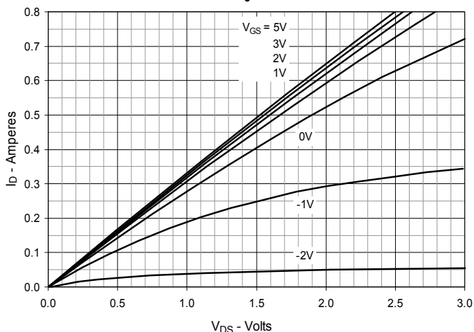
Fig. 3. Extended Output Characteristics
